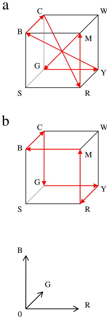
Fig.1. Two typical routes, (a) non-minimum routes and (b) minimum routes, for Type A colors (Table 1) in the RGB color space
