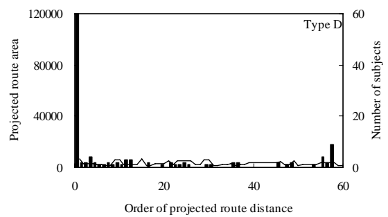
Fig.4. Relationship between order of projected route distance, route area, and number of subjects
