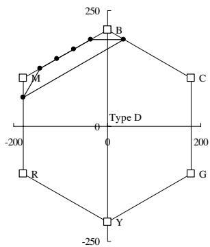
Fig.3. Projected route area on a hexagonal diagram
