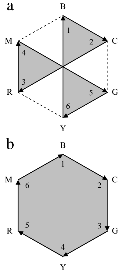
Fig.5. Two projected routes and projected route areas (shaded areas) for six fundamental colors (Type A)
